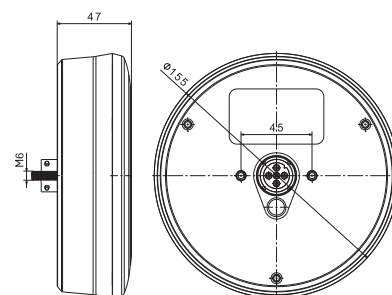
flat mounting assembly version
